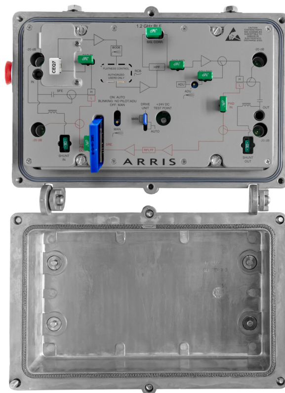
BLE with 27 dB Return Gain Shown
